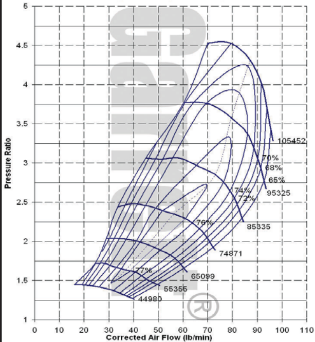
GT4202R, 102mm, 53 Trim, 0.60 A/R
