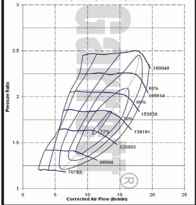
GT1548, 48mm, 60 Trim, 0.48 A/R
