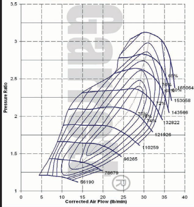
GT2860R, 60mm, 62 trim, 0.60 A/R
