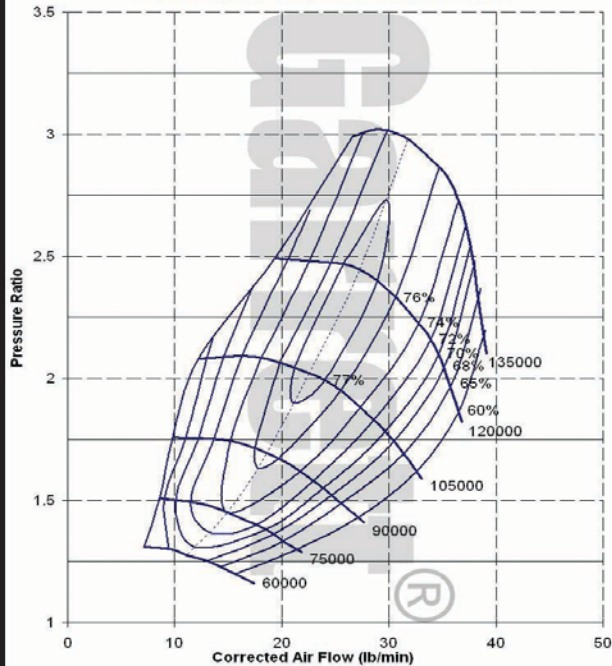
GT3271, 71mm, 52 Trim, 0.50 A/R
