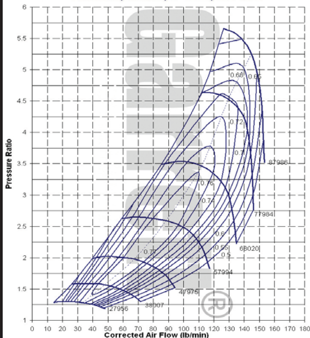
GT5533R,133mm,47 Trim,0.69 A/R
