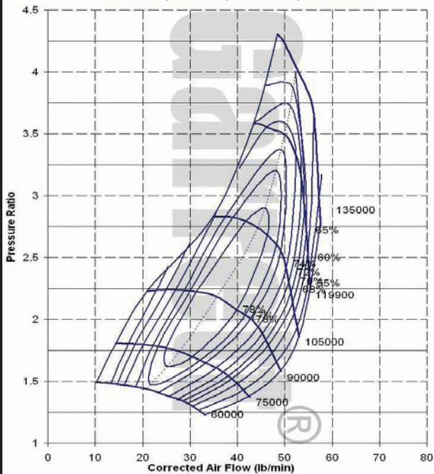
GT4082, 82mm, 50 Trim, 0.58 A/R
