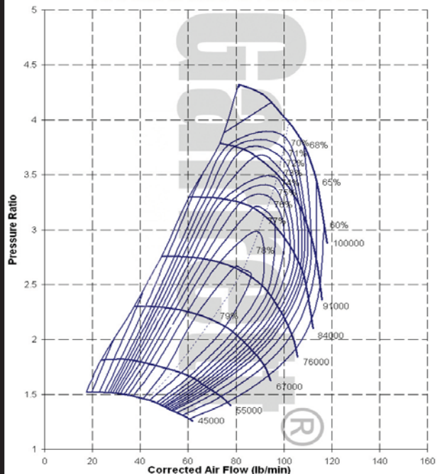
GT4708R, 108mm, 56 Trim, 0.69 A/R
