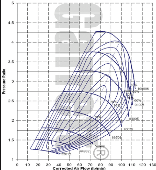
GT4508R, 108mm, 56 Trim, 0.69 A/R
