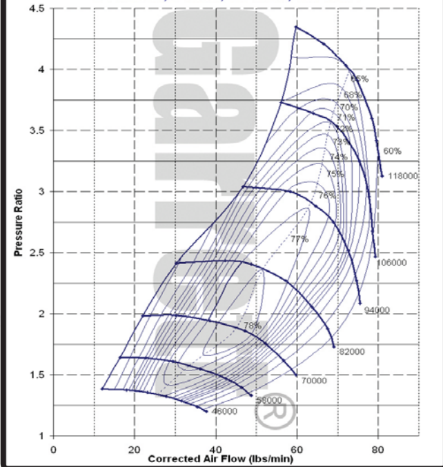
GT4094R, 94mm, 52 Trim, 0.72 A/R
