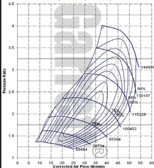
GT3076R, 76.2mm, 56 Trim, 0.60 A/R
