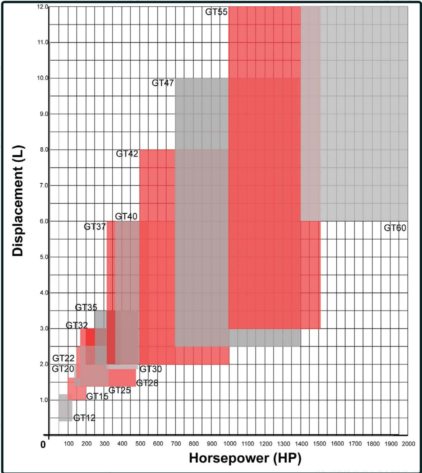
Garrett® Turbocharger Displacement Chart
